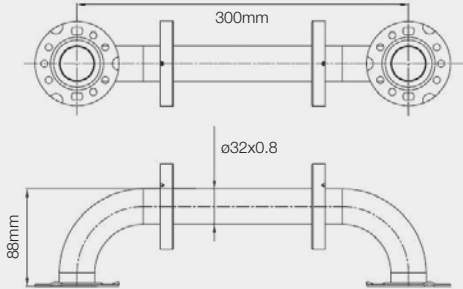
300MM GRAB BAR - 32MM Ø DIAMETER
