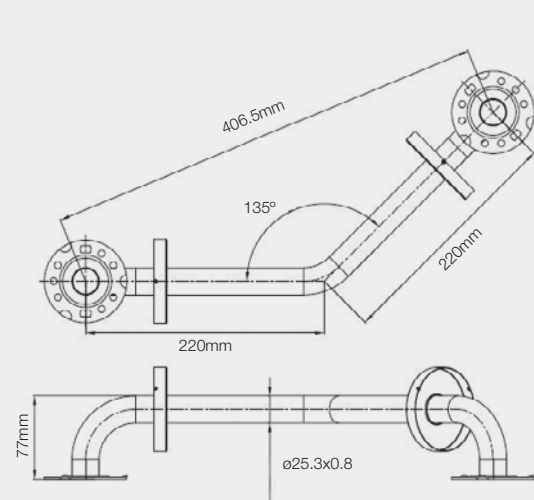
450MM ANGLED GRAB BAR - 25MM Ø DIAMETER
