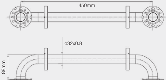
450MM GRAB BAR - 32MM Ø DIAMETER
