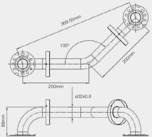
450MM ANGLED GRAB BAR - 32MM Ø DIAMETER
