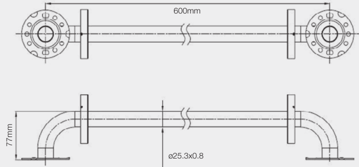
600MM GRAB BAR - 25MM Ø DIAMETER
