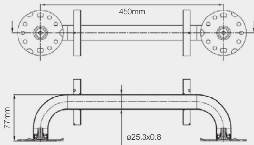
450MM GRAB BAR - 25MM Ø DIAMETER
